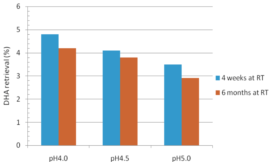
Fig 2 Influence of pH on DHA solutions (buffered with acetic acid/sodium acetate).
