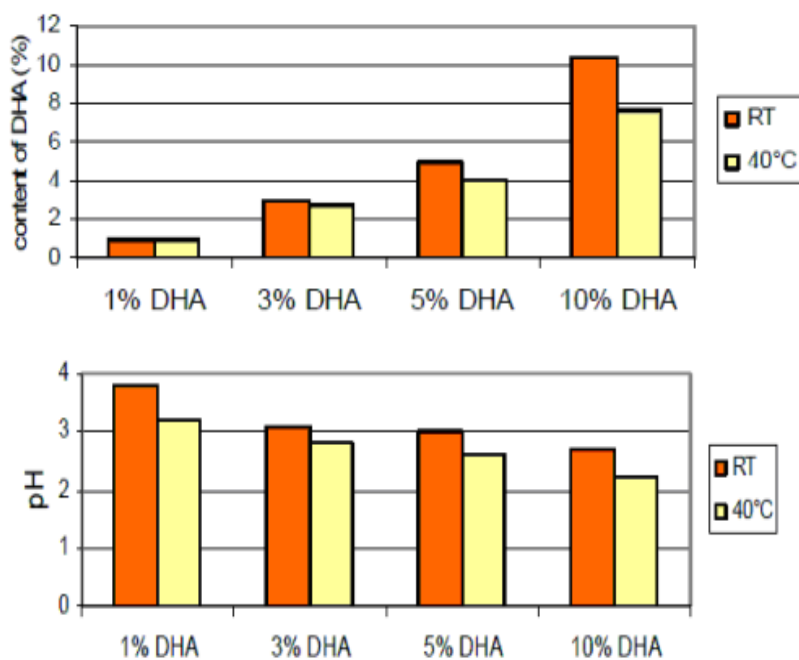
Fig 1 Stability of DHA solution after 6 months storage time (at RT and 40° C)
